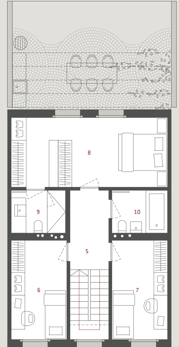
MANSARDA
