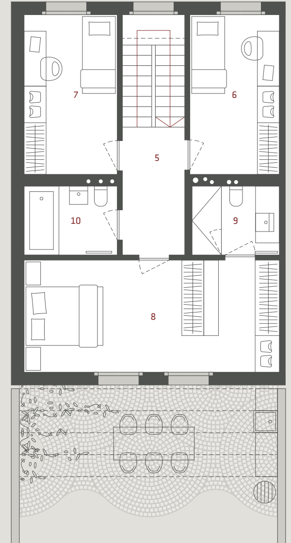
MANSARDA
